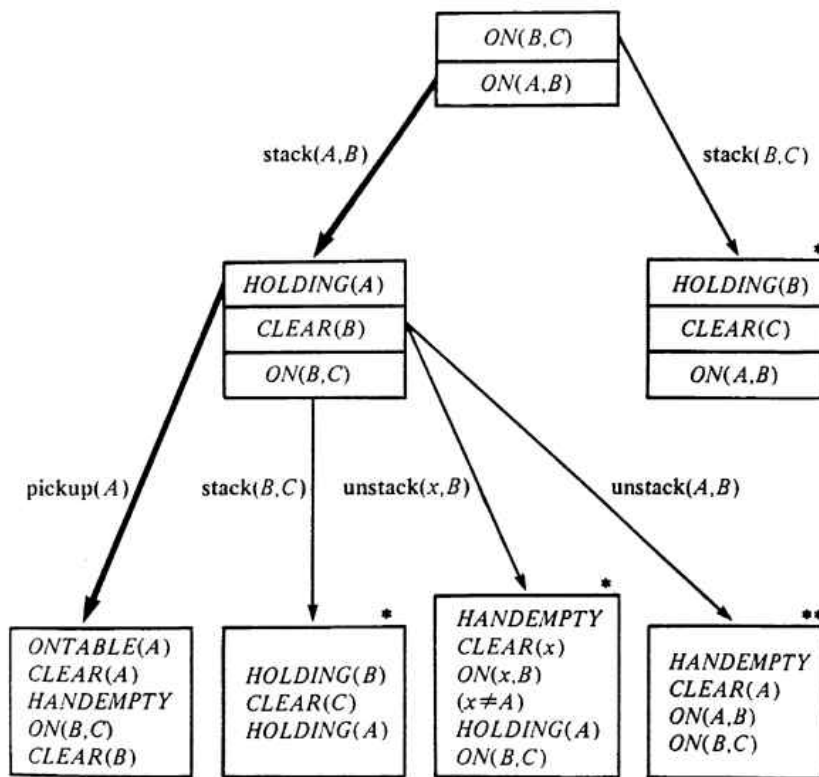
Part of the backward (goal) search graph for a robot problem.
