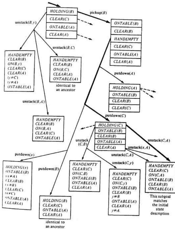
Conclusion of the backward search graph.
